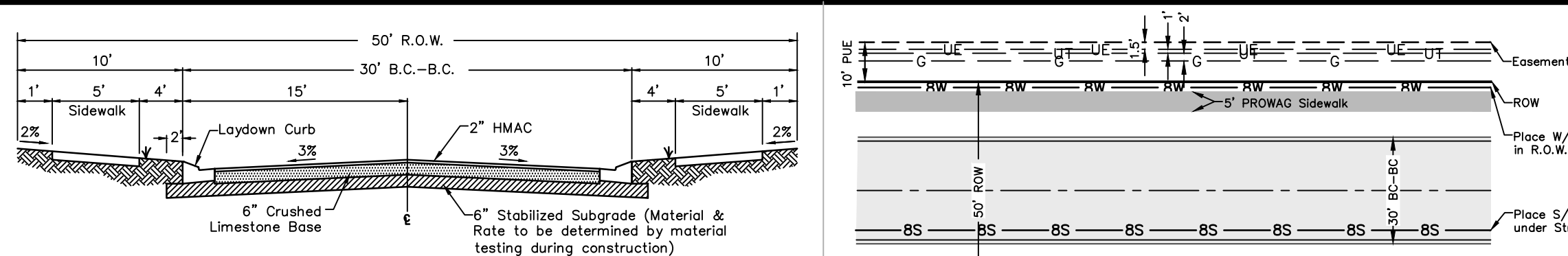
TYPICAL 30' PAVEMENT SECTION
