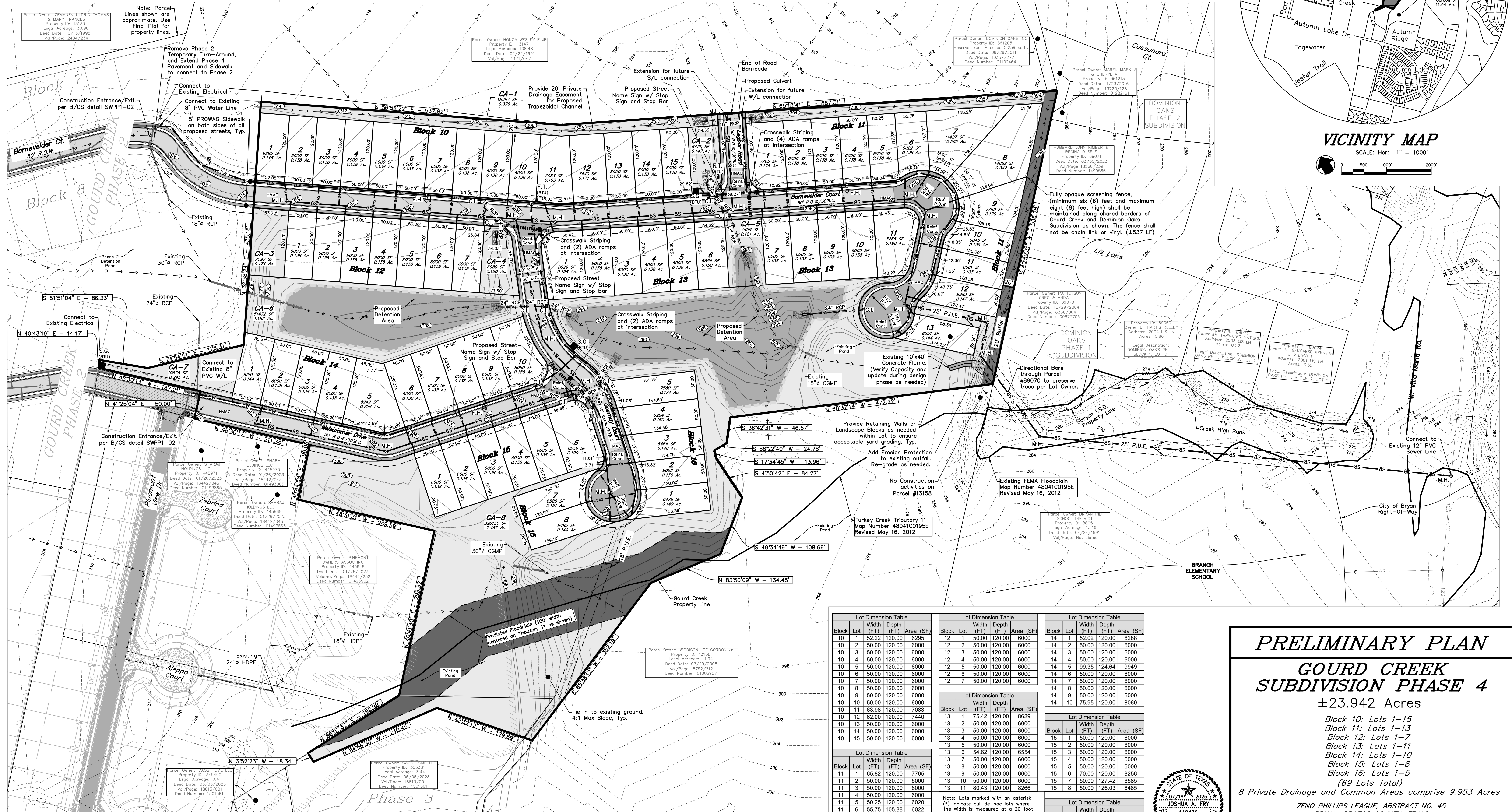
Phase 4 Preliminary Plan
