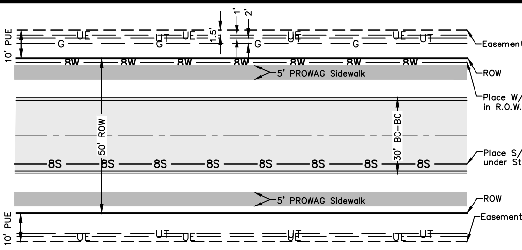
Typical Utility Layout
